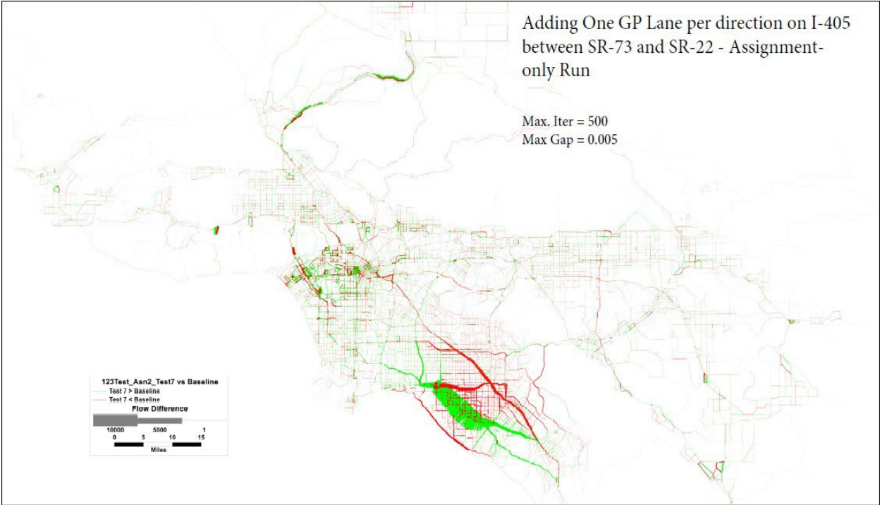
Figure 3: Volume Difference Plots with Different Assignment Convergence Criteria – Baseline plus Project vs. Baseline Assign-Only Run
